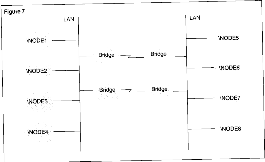
Figure 7. Expand over TLAM, coupled with one or more bridges, allows two geographically separate sites to operate as one fully interconnected network.
