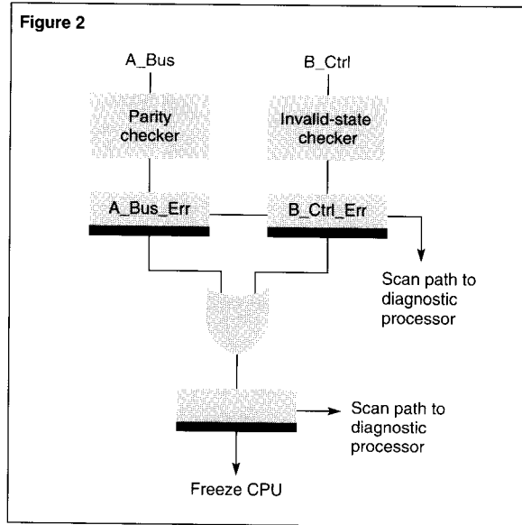
Figure 2. NonStop Cyclone error identification registers.
