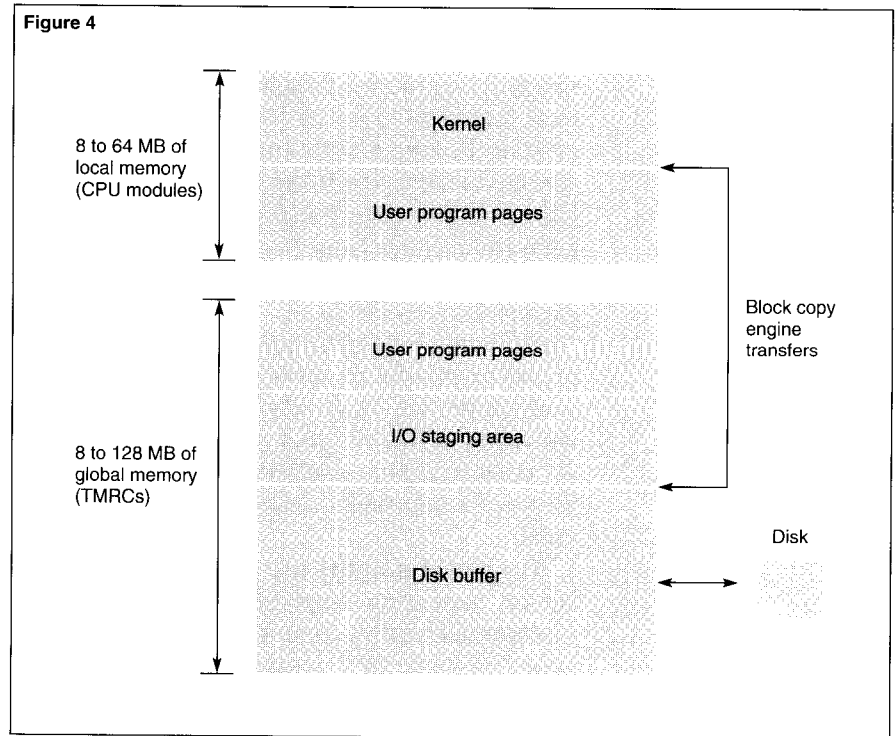
Figure 4. For optimum performance, system memory is organized in a two-tier hierarchy.
