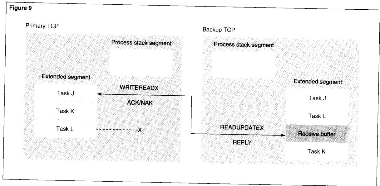
Figure 9. Step 2. The primary TCP sends checkpoint context data for Task J to the checkpoint receive buffer.
