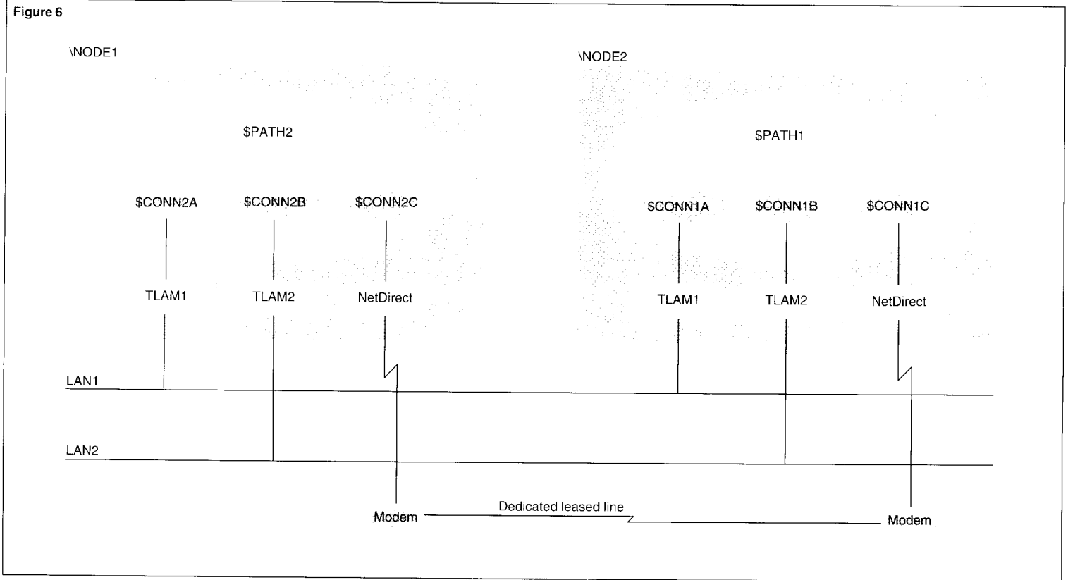
Figure 6. Extra fault tolerance is built into this configuration with the additional Expand NetDirect connection. The two Guardian 90 nodes can use NetDirect if the Expand over TLAM connections fail.
