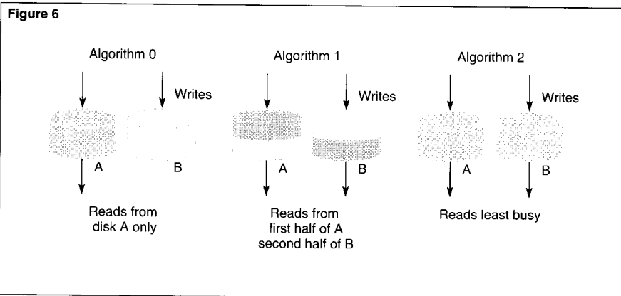
Figure 6. Read optimization of mirrored disks is a technique used to improve system performance.
