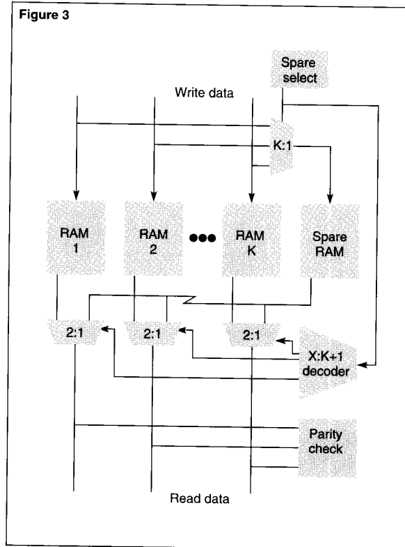
Figure 3. NonStop Cyclone spare RAM mechanism.
