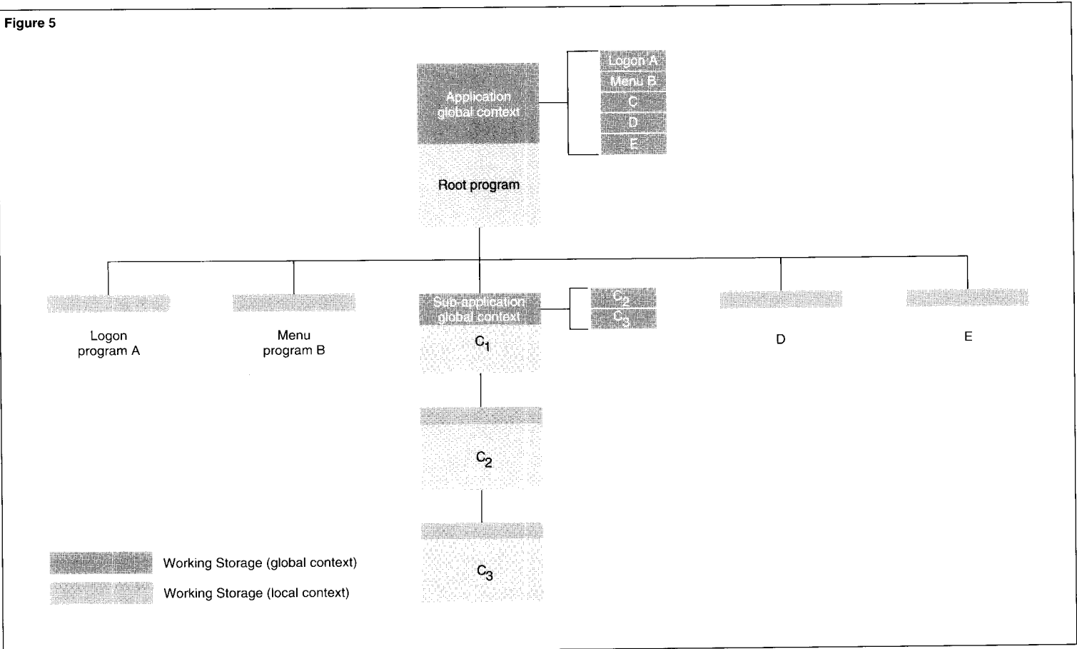
Figure 5. A combination of structured and flat application call sequences. Called programs use the application global context (shared data area) in the root program. Programs C 2 and C 3 also use the sub-application global context in program C 1 .
