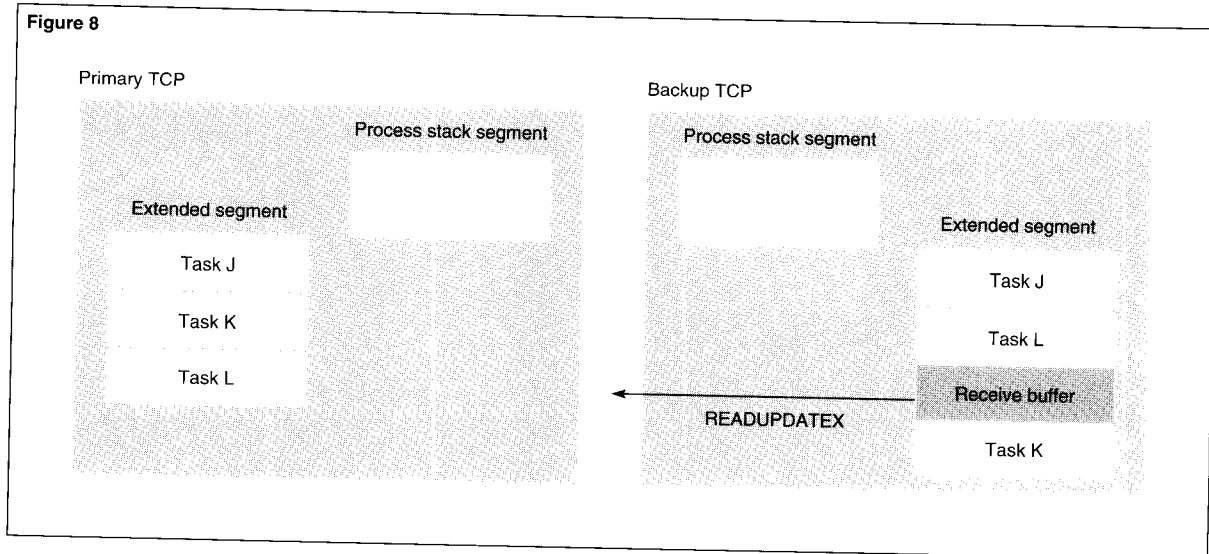
Figure 8. Step 1 of TCP task context checkpointing in the C10 and post-C10 releases of Pathway. The backup TCP allocates the extra slot as the checkpoint receive buffer.
