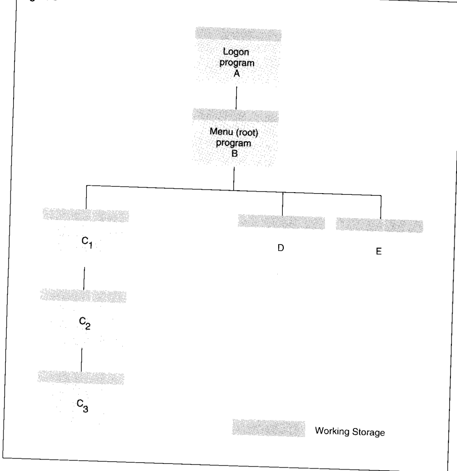
Figure 3. A structured application call hierarchy.
