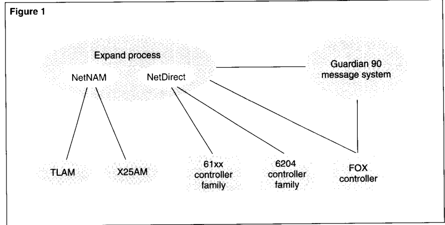
Figure 1. The connectivity options available for Expand.
