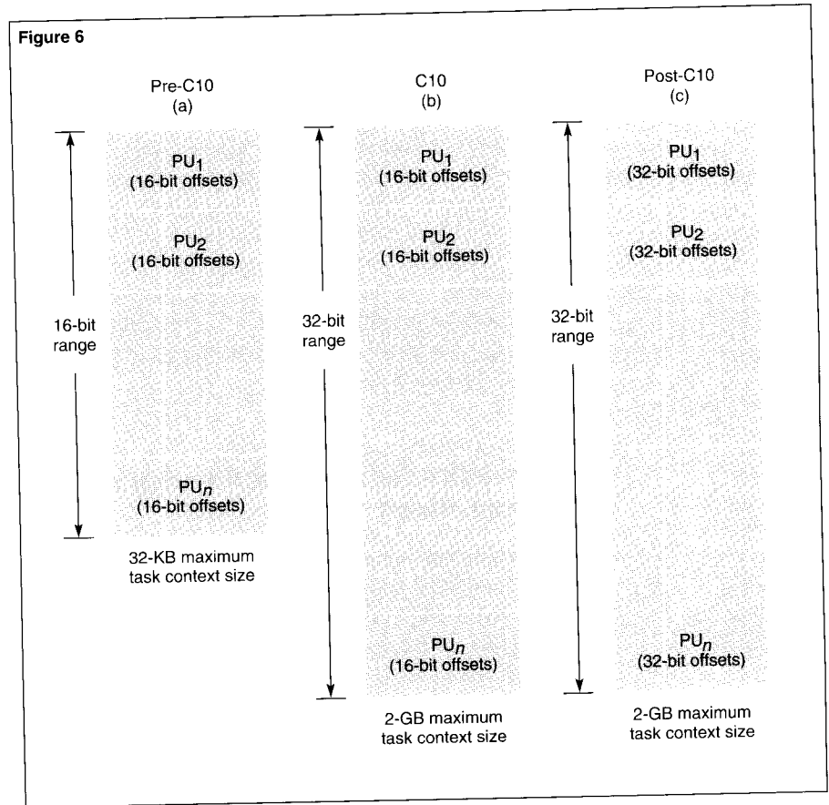
Figure 6. Relationship of program unit (PU) size and task context size.
