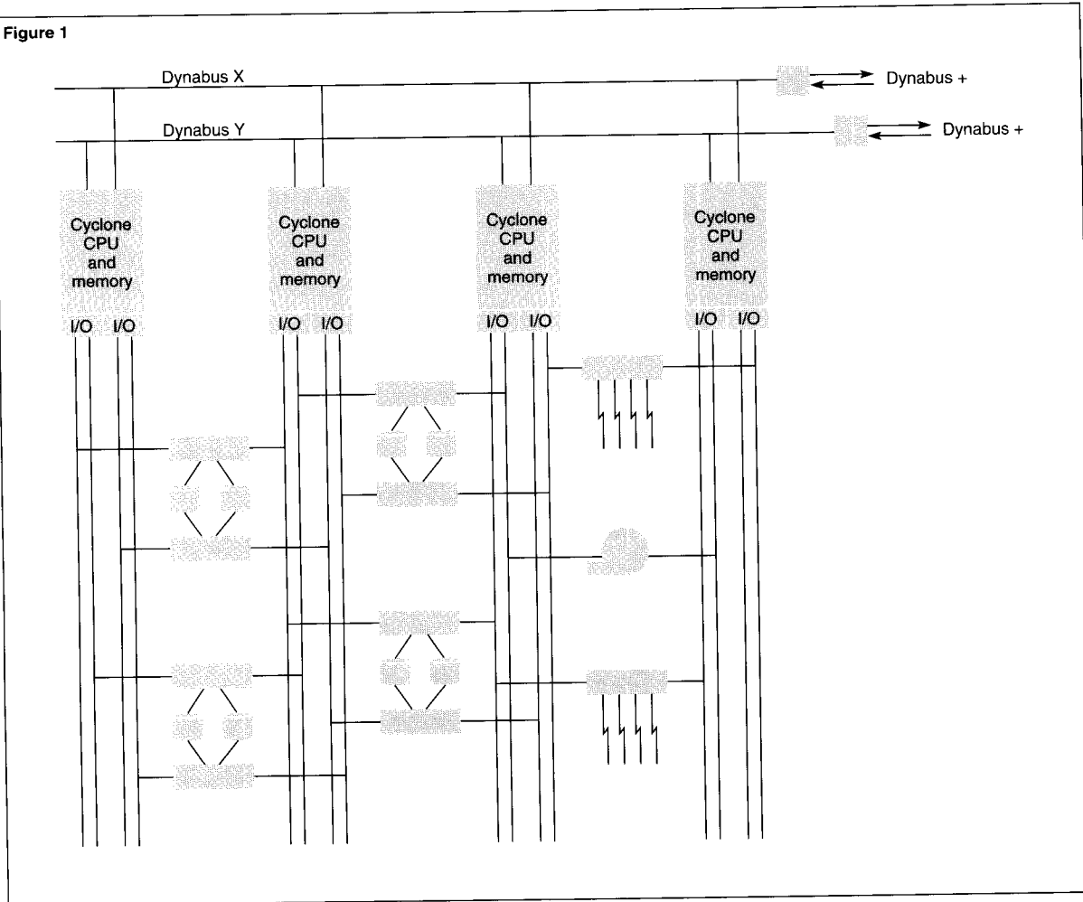
Figure 1. NonStop Cyclone system architecture.
