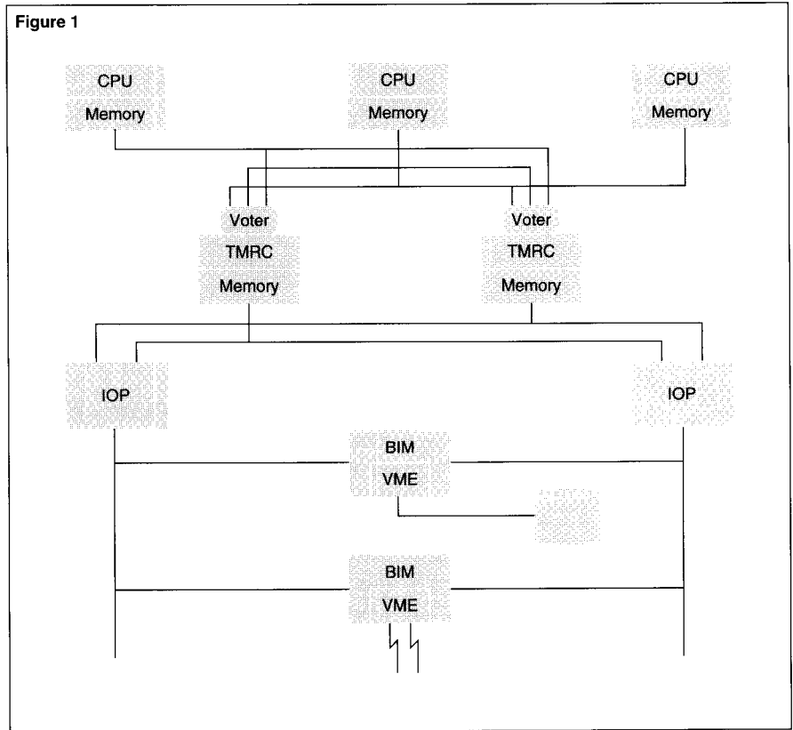
Figure 1. The Integrity S2 hardware architecture uses a triple modular redundant design with replicated components and data paths.
